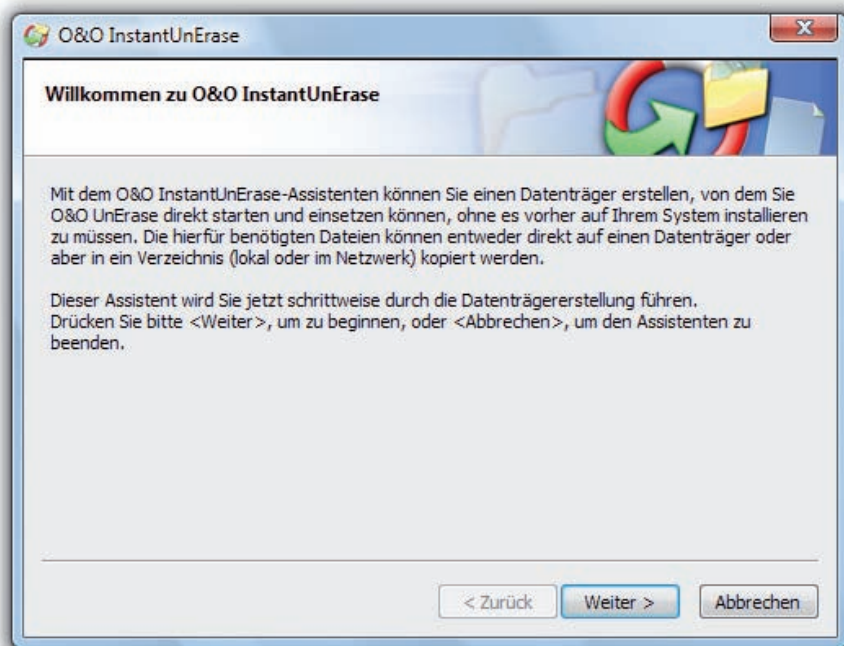
O&O- InstantUnErase-Assistent
